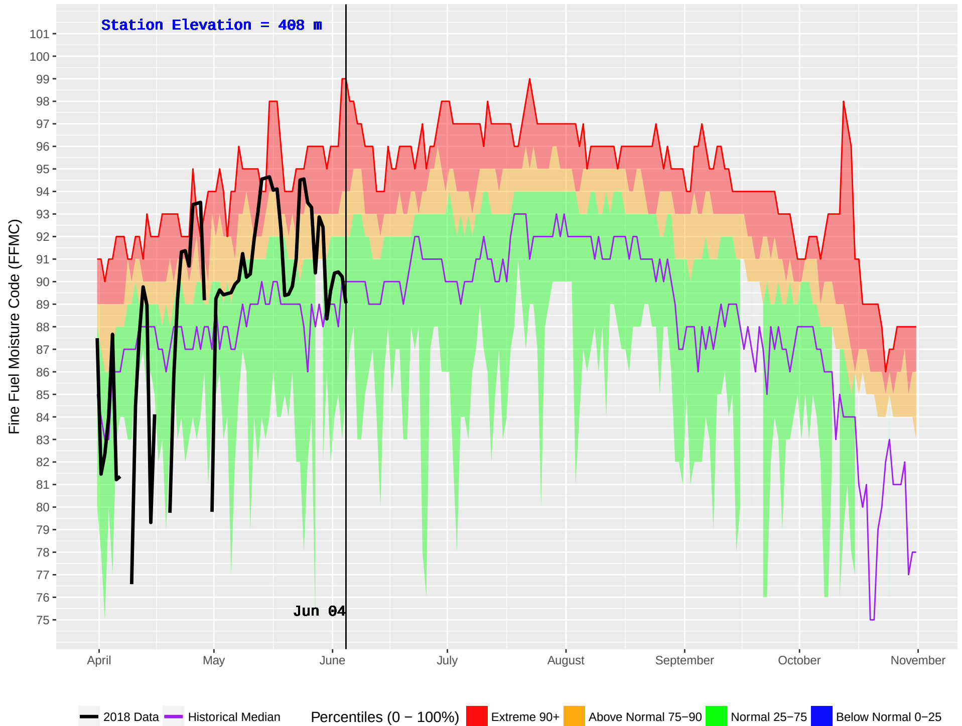
LILLOOET (280) : Historical (1977–2016) and Current (2018) Noon Fine Fuel Moisture Code (FFMC)
